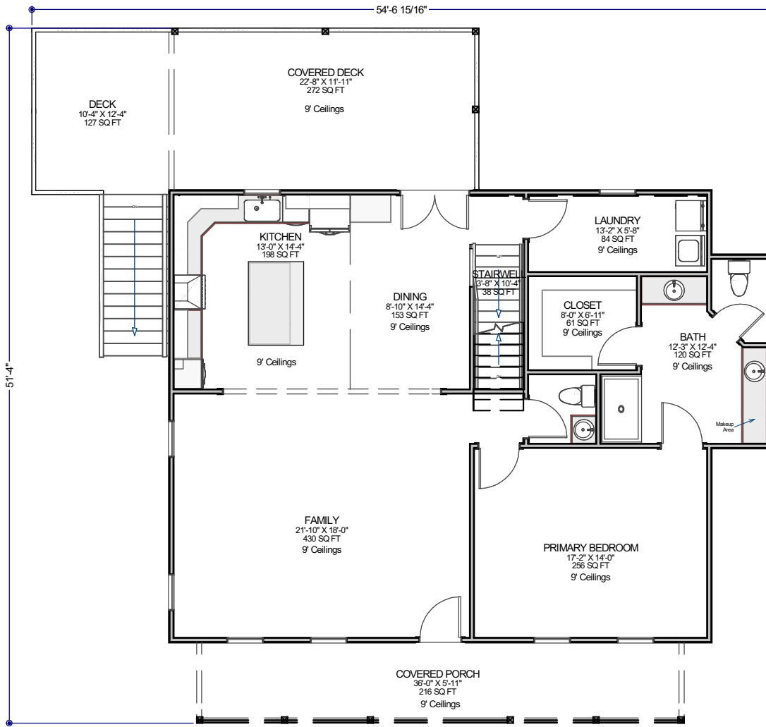
1st Floor
