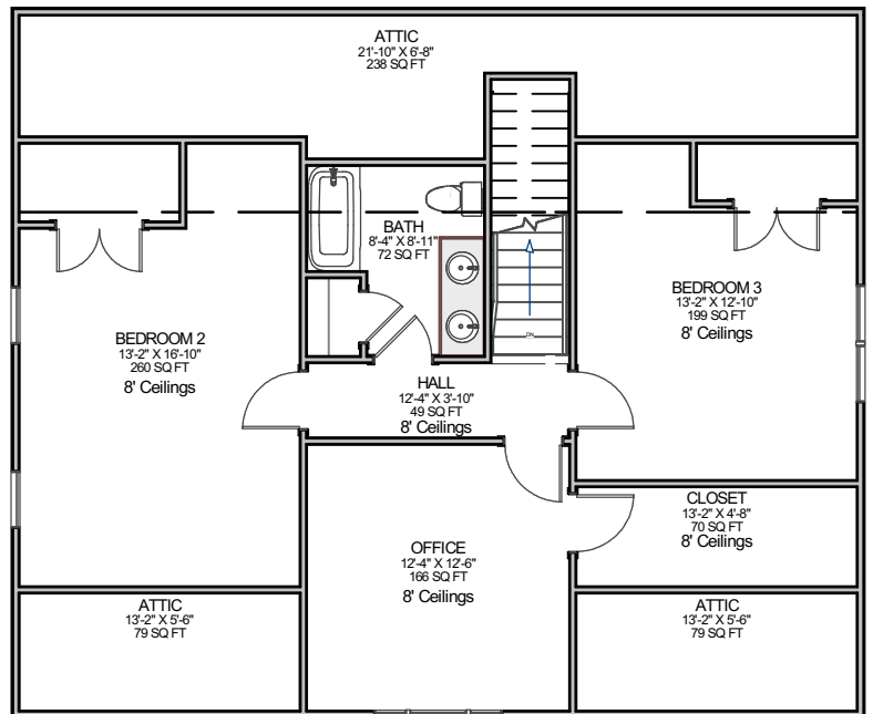
2nd Floor
