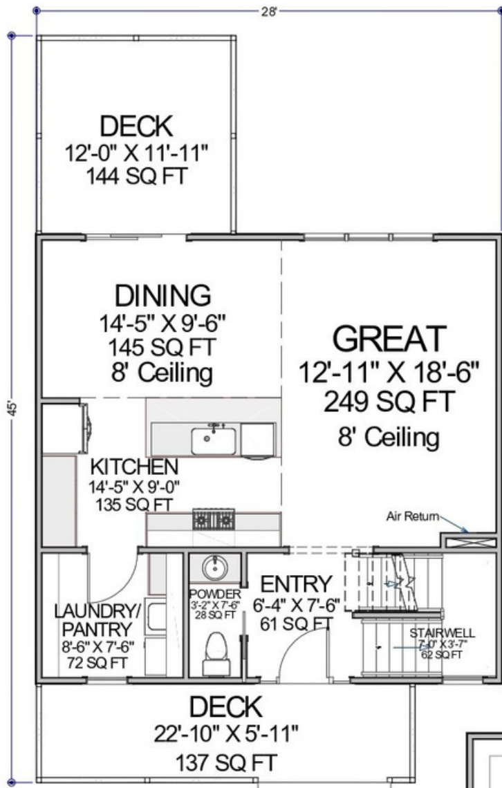
1st Floor
