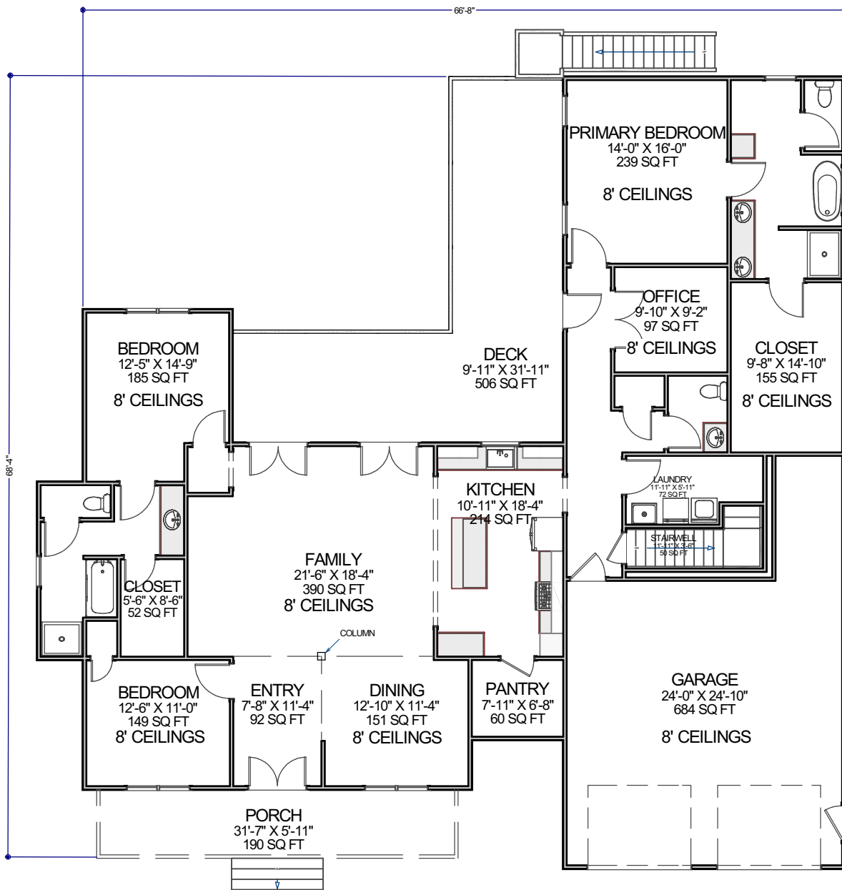
1st Floor
